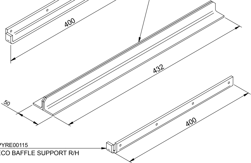
PYREAC478 ECO BAFFLE SUPPORT MIDDLE
