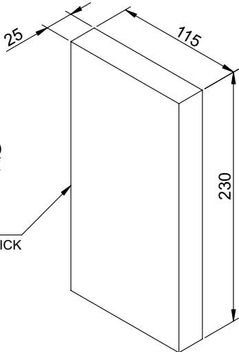
PYRE00355 ea (2 req'd) CERAMIC BRICK
