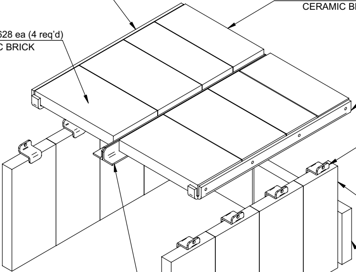
PYREAC478 ECO BAFFLE SUPPORT MIDDLE
