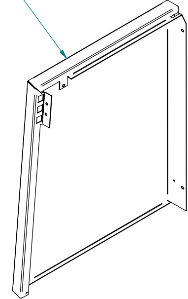
JAY-SFSE00006 SIDE PANEL L/H
