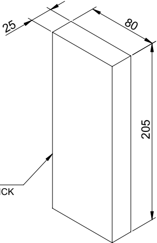
PYRE00116 ECO BAFFLE SUPPORT L/H
